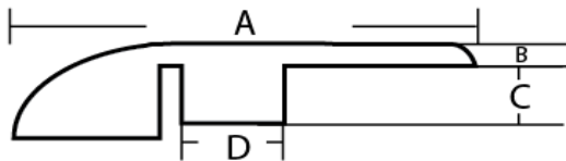
Reducer (2400mm)
