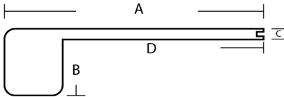
Square Edge Flush Stairnose - 60"(1524mm)
